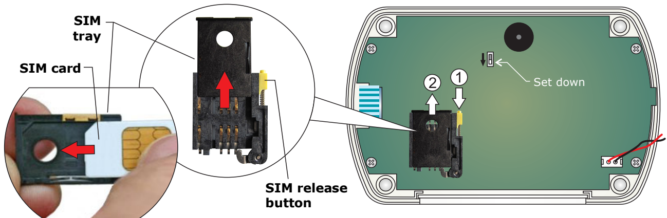
Fig. 6.8.1: inserting the SIM card
