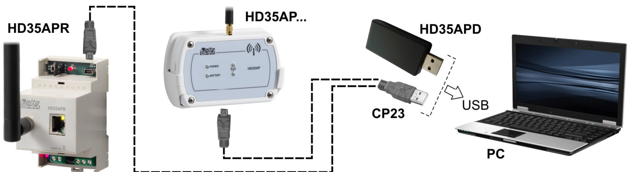
Fig. 6.4.1: USB connection
