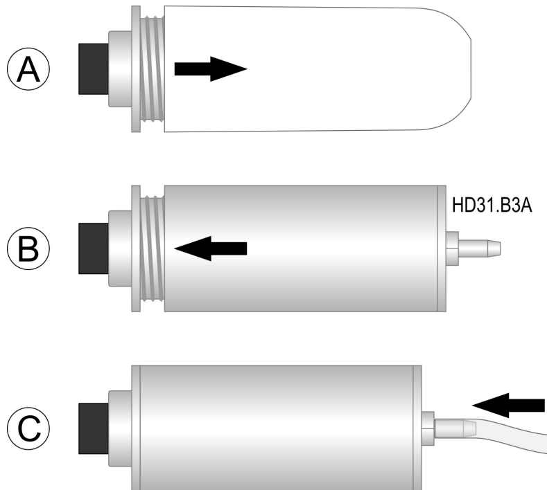
Fig. 9.7.1: CO 2 calibration with nitrogen cylinder
