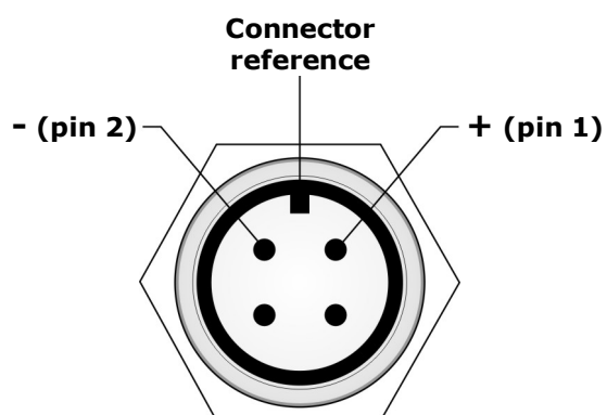
Fig. 9.8.1: external view of the instrument M12 connector
