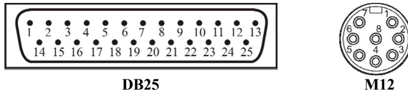
Fig. 39 - HD2110CSM cable connector pin numbers
