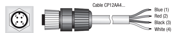
M12 male connector of the transmitter
