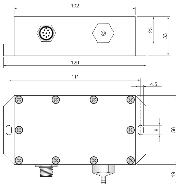
Fig. 1: dimensions (mm)
