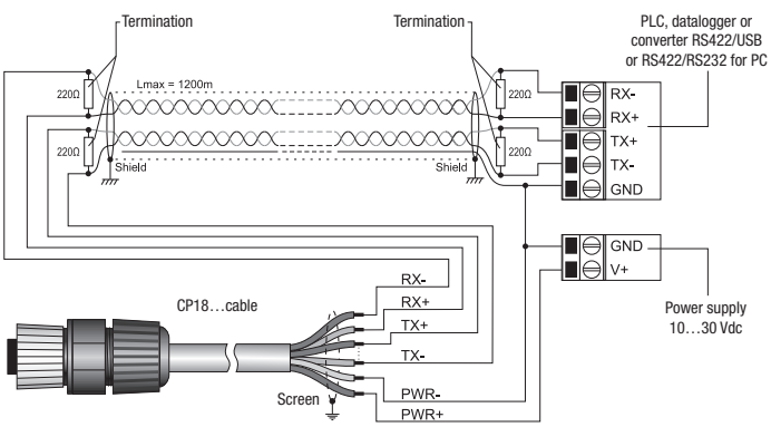
Fig. 4: RS422 connection
