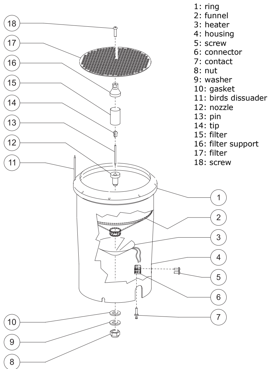
Fig. 10 – Exploded view of the upper part (version with heating)
