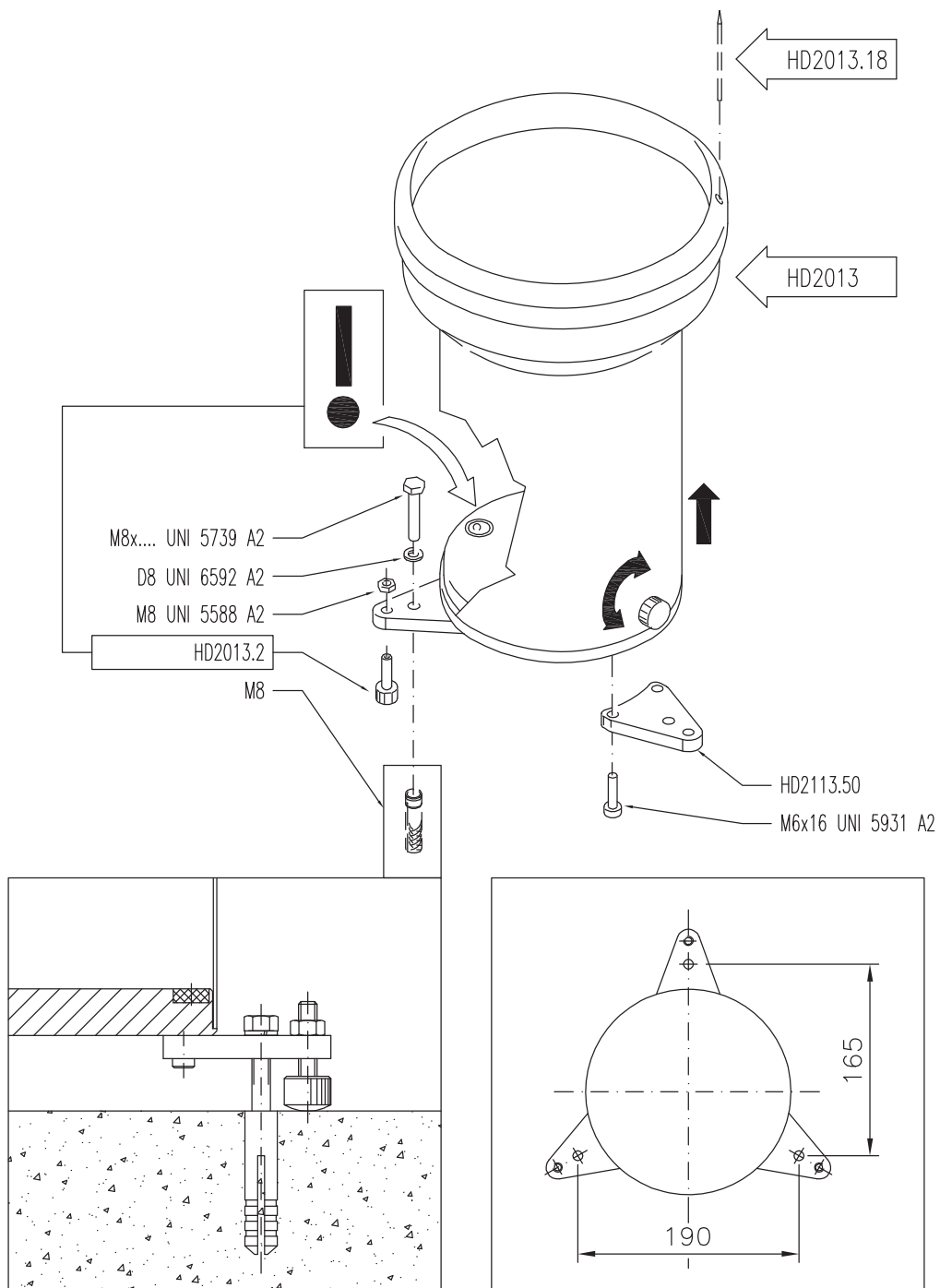
Fig. 11 – Ground installation
