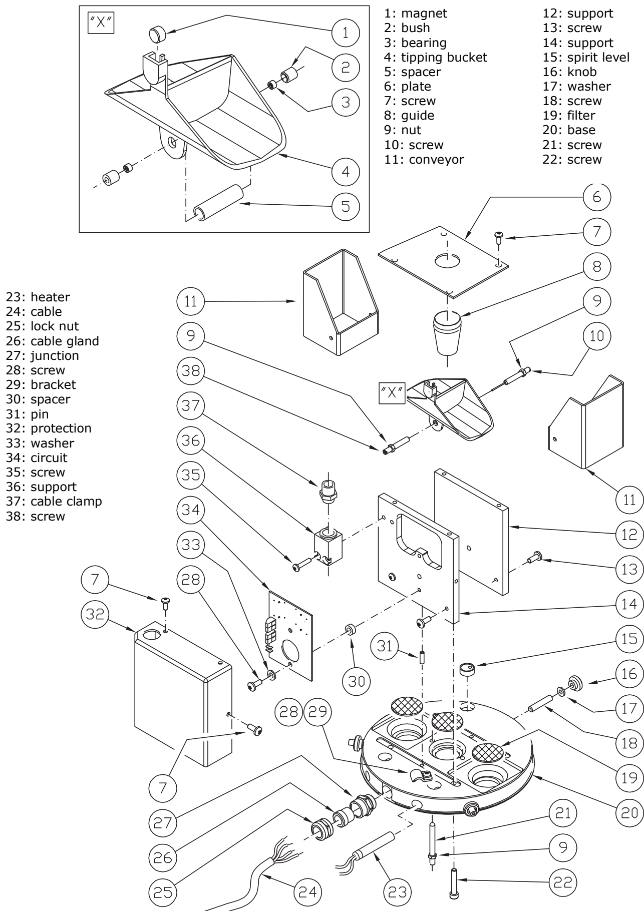
Fig. 14 – Exploded view of the lower part (version with heating)
