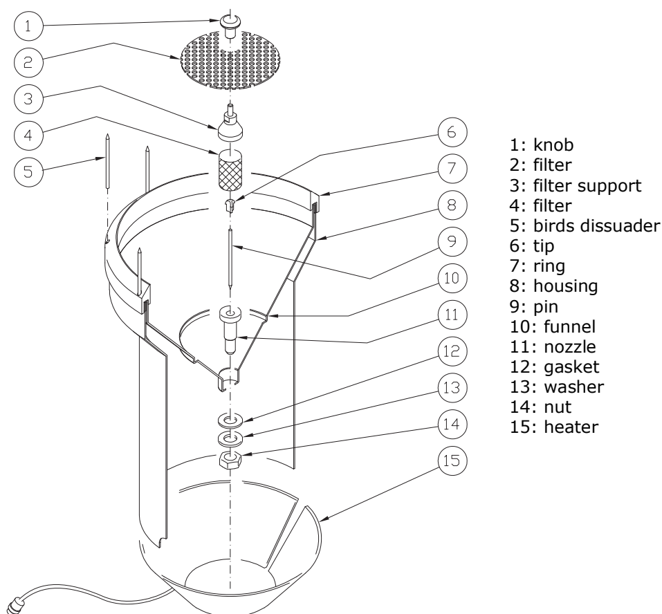
Fig. 13 – Exploded view of the upper part (version with heating)
